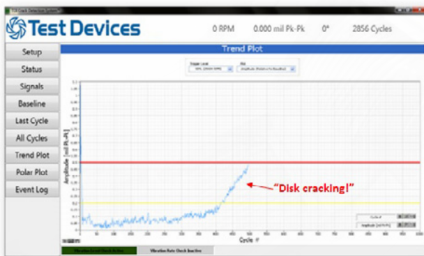
Figure-5: Example of Real-Time Crack Detection data.
