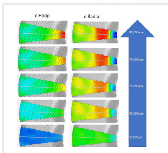
Figure-4: An example of full-field strain mapping test result.
